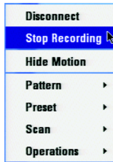
Figure 34. Stop Recording
